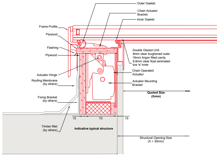
Sectional Drawings
